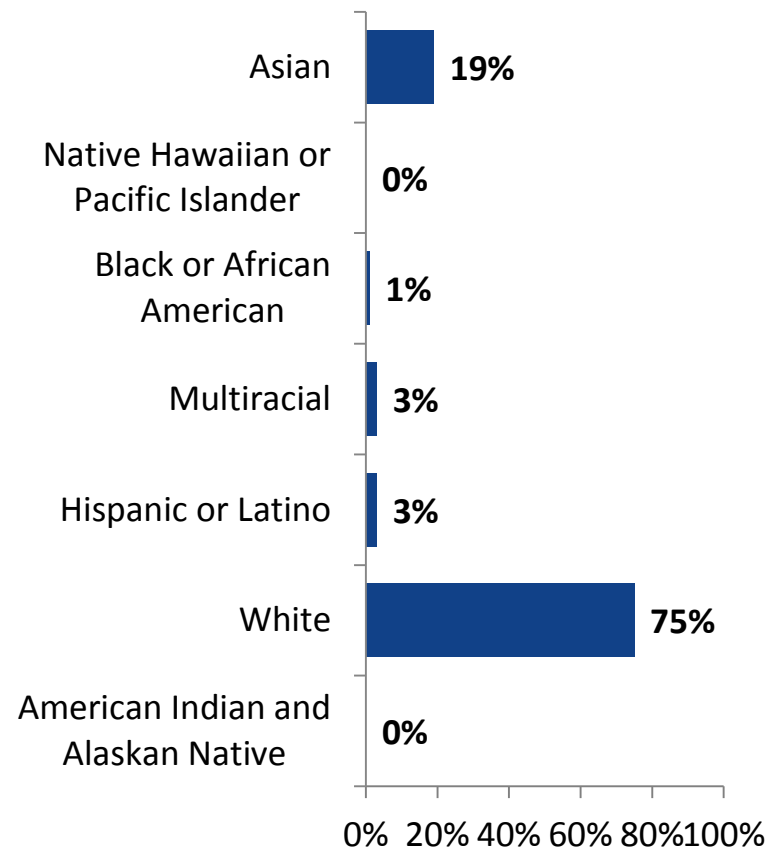
Parents (N=272)
