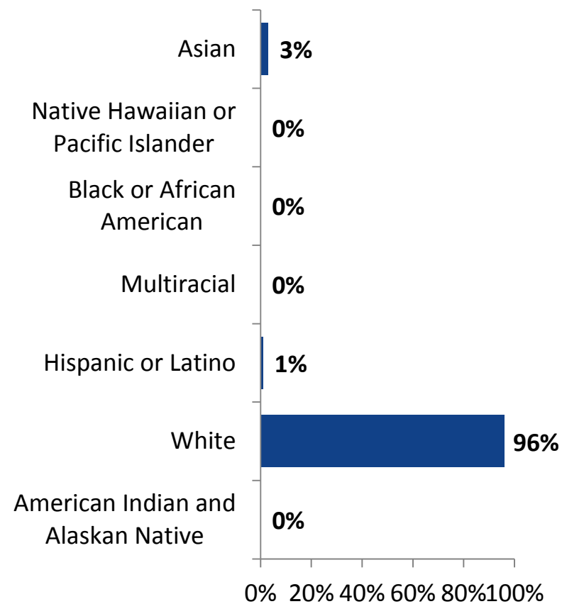
Staff (N=70)
