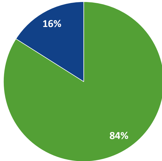
Parents (N=275)
