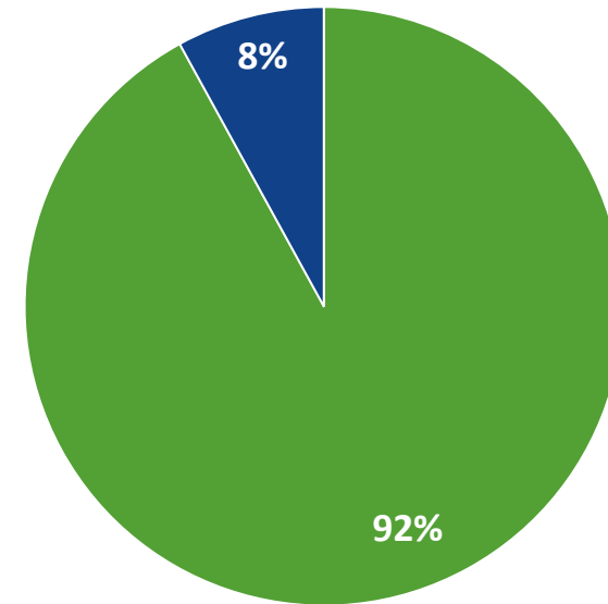
Staff (N=74)
